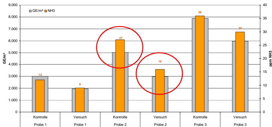
Geruchsemission vs. Ammoniak Durchgang 1
