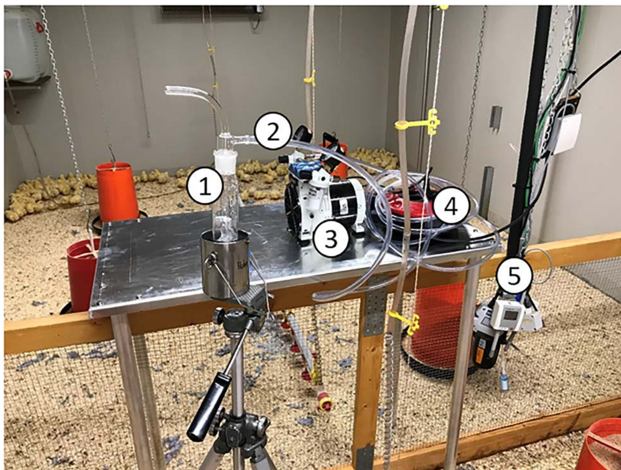
Figure 1. Sampling device used inside the chicken barn (1) ACE Glass impinger, (2) vacuum tube, (3) pump, (4) power source, and (5) sensors for gases and humidity). The impinger is connected to a pump powered by electricity. Simultaneously, gases, temperature, and humidity are recorded during air sampling.
