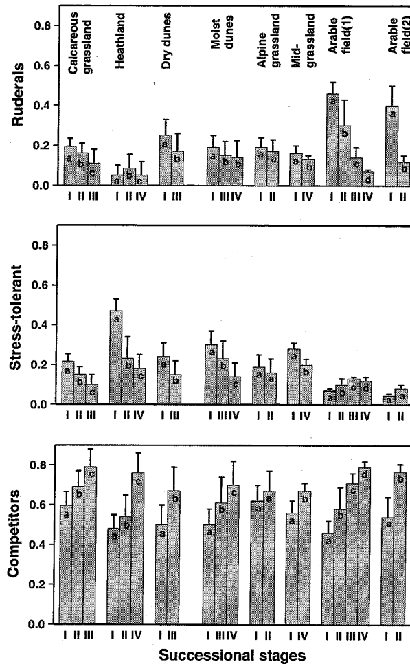
Fig. 4 Plant strategies according to Grime's classification. We present average plot values for competitiveness (C), stress-tolerance (S) and ruderal type (R) for the different stages of succession. For a given habitat, different lowercase letters indicate statistical differences among stages ( P < 0.05 ). Bars indicate standard deviations
