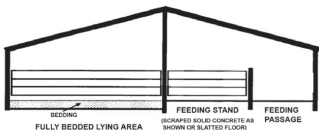
Figure 3.8.5.1.1: bedded house with concrete feeding stand.
