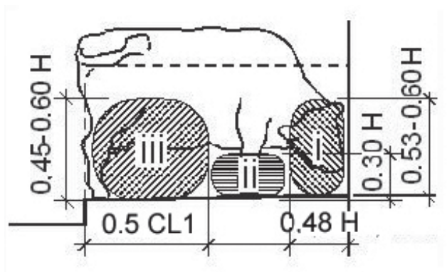
Figure 3.1.2.4.1: three zones of freedom in cubicles. (Note: H = Height at withers).
