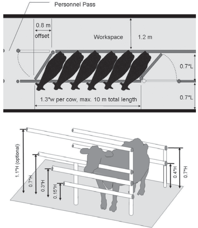
Figure 3.10.6.1: dimensions of palpation rail unit shown by plan and side view, respectively (after MWPS, 7 th edition, 2013).
