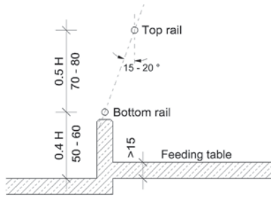
Figure 3.3.4.1.1: post & rail barrier dimensions. The dimensions are only appropriate for dehorned cows.
