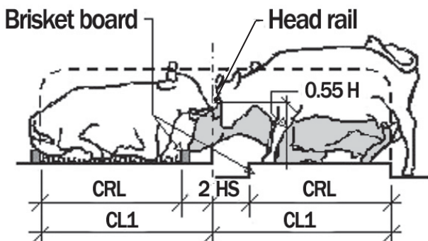
Figure 3.1.2.4.2: head to head cubicles with front space sharing.
