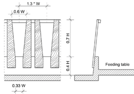
Figure 3.3.4.4.1: dovetail barrier, construction details.
