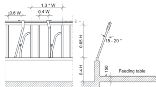
Figure 3.3.4.5.1: typical self locking barrier.
